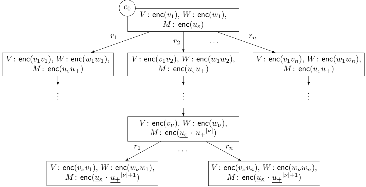
Figure 2: The canonical model \mathcal{I}_{\mathcal{P}} for an instance \mathcal{P} of the PCP
