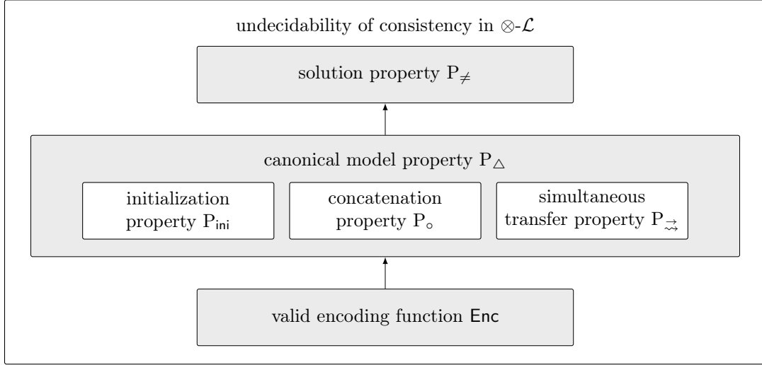
Figure 4: A new way to prove the canonical model property
