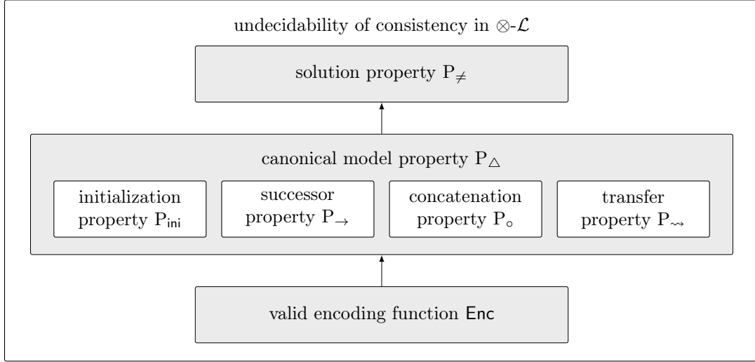
Figure 3: The framework for showing undecidability of consistency in a fuzzy DL \otimes\text{-}\mathcal{L}
