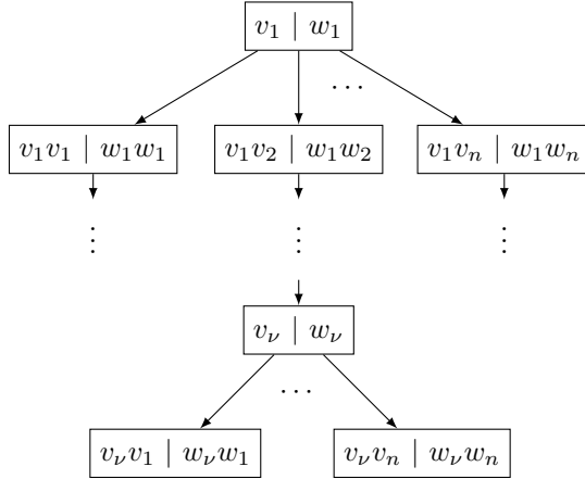
Figure 1: The search tree for an instance \mathcal{P} of the PCP
