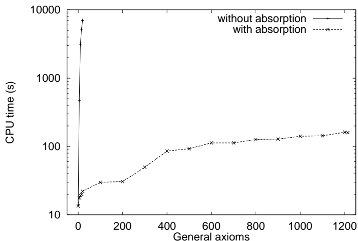
Figure 1: Classification times with and without absorption
