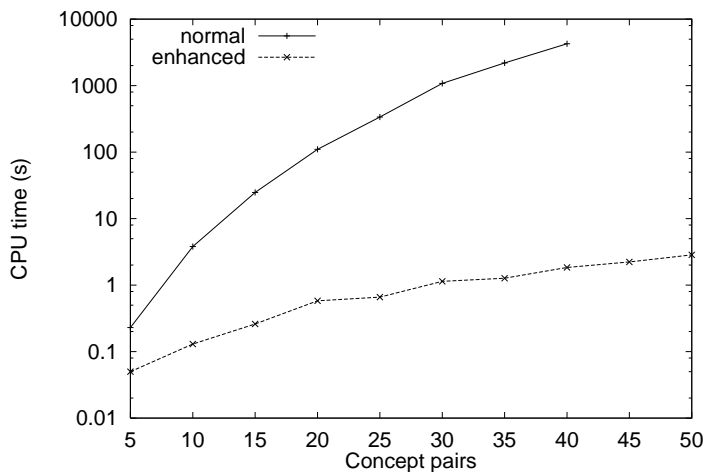
Figure 2: Classification times with and without enhanced absorption
