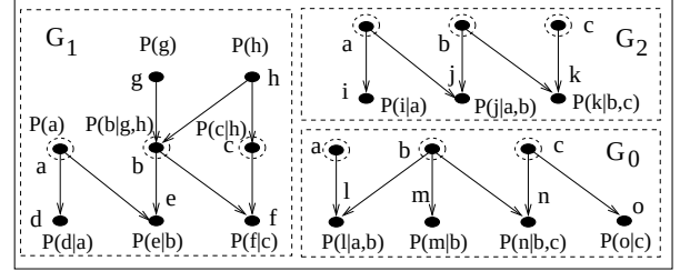
Figure 1: A trivial MSBN where each d-sepnode is shown with a dashed circle. The hypertree has the structure G_1 - G_0 - G_2 and each d-sepset is \{a, b, c\} .
