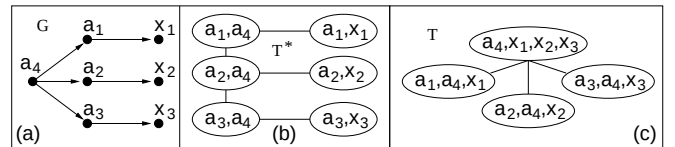
Figure 4: (a) Subnet G . (b) The JT T^* from G by unconstrained triangulation. (c) The JT T from triangulation constrained by \{x_1, x_2, x_3\} .
