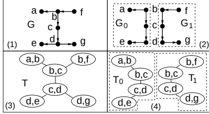
Figure 3: Illustration of natural subdomain disruption.
