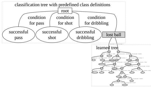
Figure 8: Classification tree. To classify the ball actions into different action classes we use a classification tree consisting of defined conditional leafs for successful actions and a learned decision subtree for lost balls.
