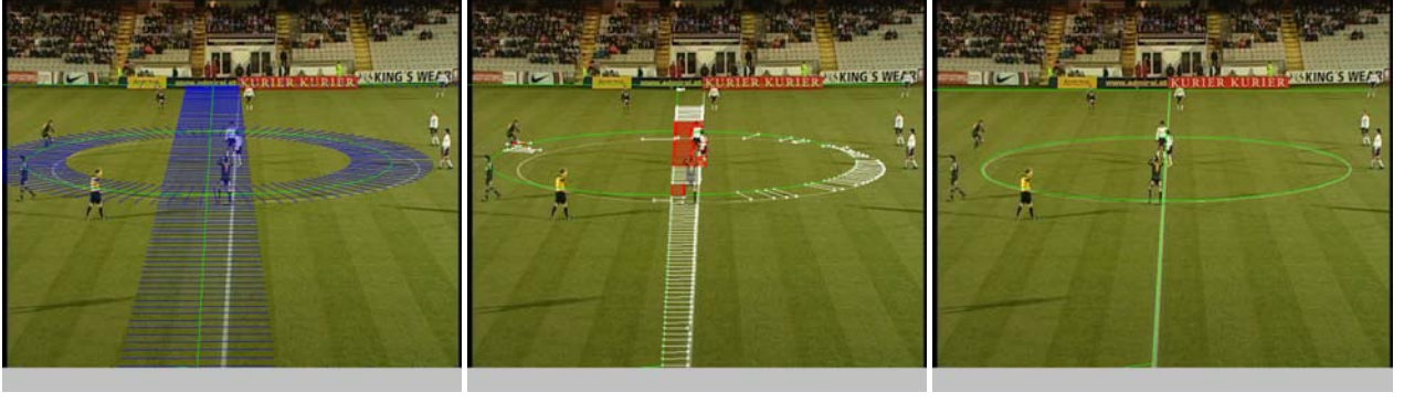
Figure 5: Estimating the camera parameters by taking the current parameters, projecting the field model using the current parameters onto the image (left), finding the correspondences between model points and the imagepoints (middle), and adjusting the camera parameters to achieve minimal errors (right).
