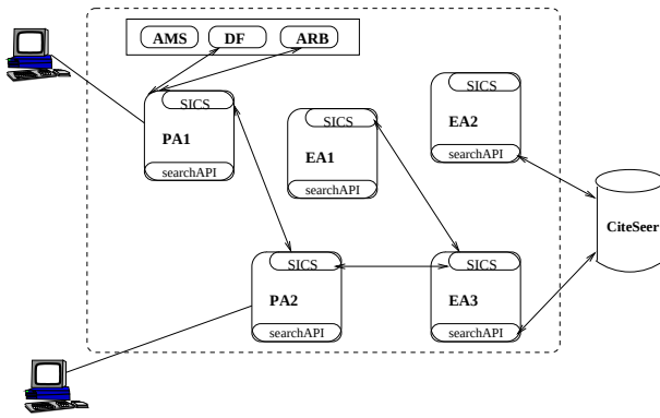
Figure 2: The architecture of a single system node. Users of the system node query their personal agents on the platform. Personal agents contact one another to find papers on a specified topic. They also use a search API to contact different information providers, e.g. CiteSeer. A SICS module inside the personal agent filters and re-ranks collected information. There are also expert agents running on the platform, which are the clones of the personal agents of the experts on the topic.
