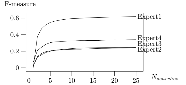
Figure 7: Average F-measure of 10 simulations with different number of searches.
