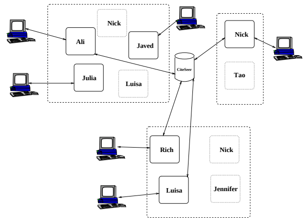
Figure 1: An example of several platforms with three ad hoc communities. Cloned expert agents are depicted with dotted squares. Julia, Ali and Javed also form an organizational community.
