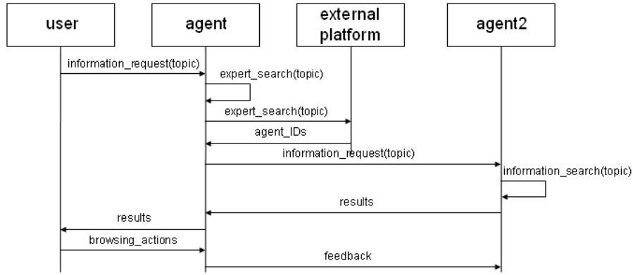
Figure 4: Sequence diagram in response to an information request.
