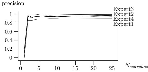
Figure 5: Average precision of 10 simulations with different number of searches.
