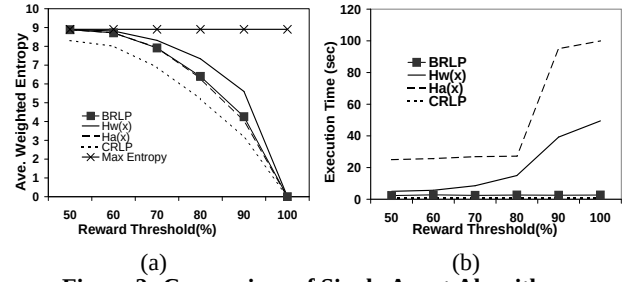
Figure 2: Comparison of Single Agent Algorithms
