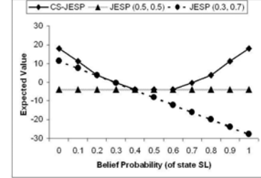
Figure 5: Comparison of the expected values obtained with JESP for specific belief points and CS-JESP
