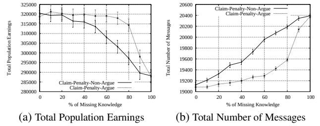
Figure 3: Efficiency and Effectiveness of the Argue and Non-Argue strategies with 20 Agents and 3 Roles.
