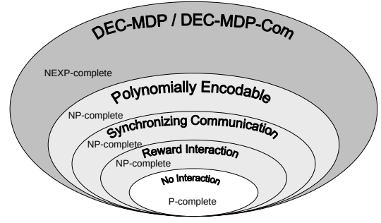
Figure 1: The relationships and complexity between various distributed MDP models.
