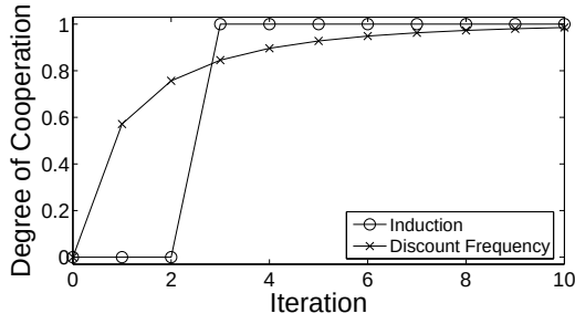
Figure 2: Learning speeds of the induction method and the discounted frequency method when the other player always cooperates. The initial degree of cooperation is zero, the discount rate is 0.75, and the promotion threshold is 3.
