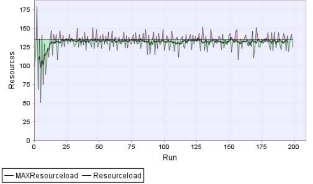
Figure 6: Development of server load for 200 cycles with resource limit of 135 units.
