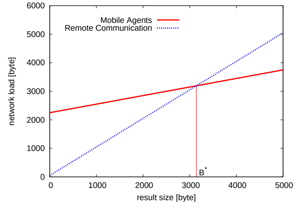
Figure 1: Evaluation of a simple mathematical model with [kB] B_{req} = 50 , B_c = 2000 , B_s = 100 , \varsigma = 0.7 and break-even point B^* \approx 3143
