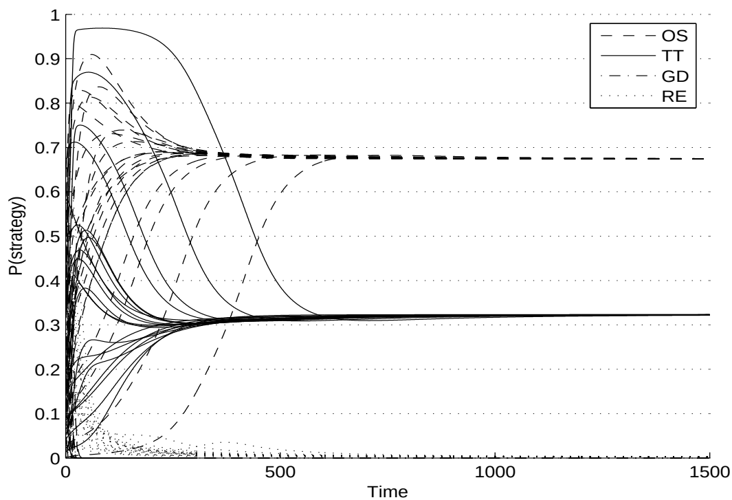
Figure 6: Replicator dynamics time series plot for a 12-agent clearing-house auction showing interaction between optimised strategy (OS) versus GD, TT and the original Roth-Erev strategy (RE)
