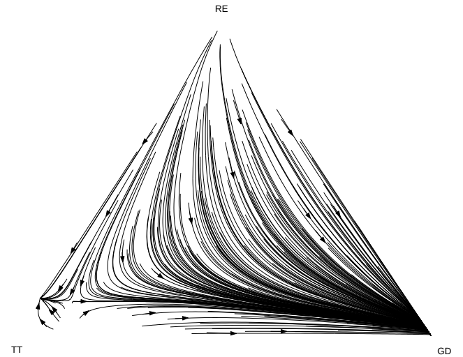
Figure 1: The original replicator dynamics direction field for a 12-agent clearing-house auction with the original unoptimized Roth-Erev strategy (labelled RE).
