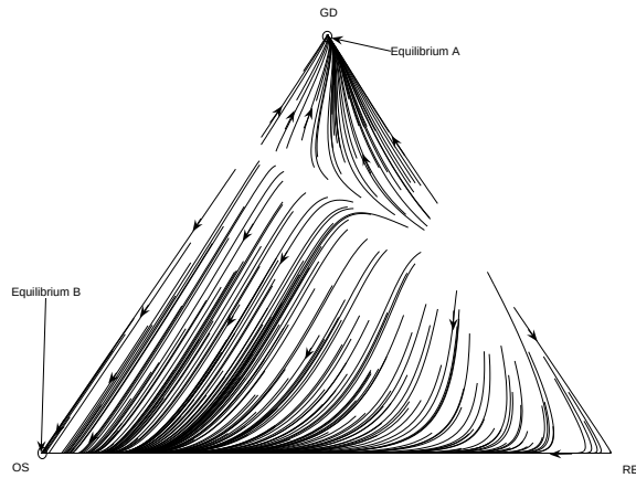
Figure 4: Replicator dynamics direction field for a 12-agent clearing-house auction showing interaction between optimised strategy (OS) versus GD and the original Roth-Erev strategy (RE)
