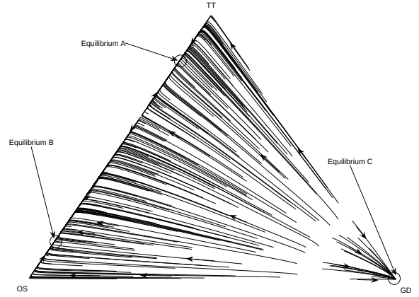
Figure 3: Replicator dynamics direction field for a 12-agent clearing-house auction showing interaction between optimised strategy (OS) versus TT and GD
