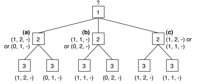
Figure 2: Example search tree in Spades.
