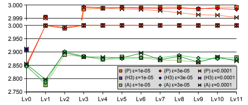
Figure 4: Average pay-off after learning with various \varepsilon values. Pay-off is averaged for 5 \times 10^8 steps after 5 \times 10^8 learning. The upper graph enlarges the top part of the lower graph.
