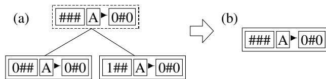
Figure 4. Integration method; (a) sub-tree after some adjust; (b) an integrated schema substitutes the sub-tree.
