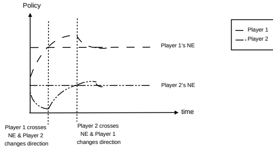
Figure 3: An illustration of WPL convergence.
