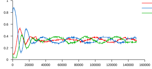
(a) GIGA-WoLF, \alpha = 0.1
