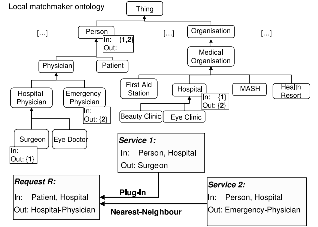
Figure 2: Example of hybrid service matching with OWLS-MX
