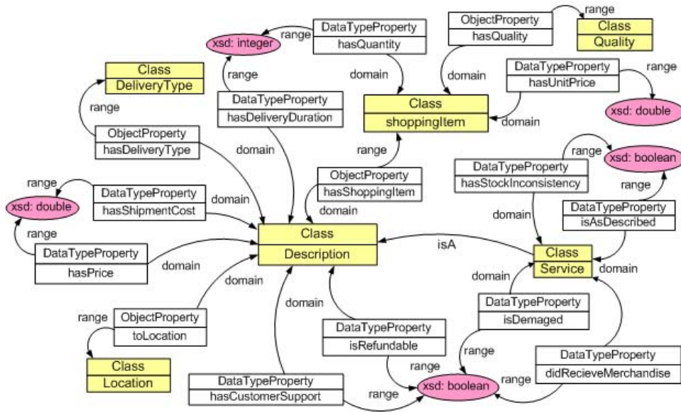
Figure 3: Domain level ontology for online shopping.
