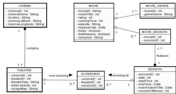
Fig.2 – A UML Class diagram detailing attributes for entities associated with the cinemaAssistant rule.
