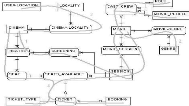
Fig.1 – Normalized Entity Relation Diagram Modeling the Cinema Problem, with four Logic Flow Lines
