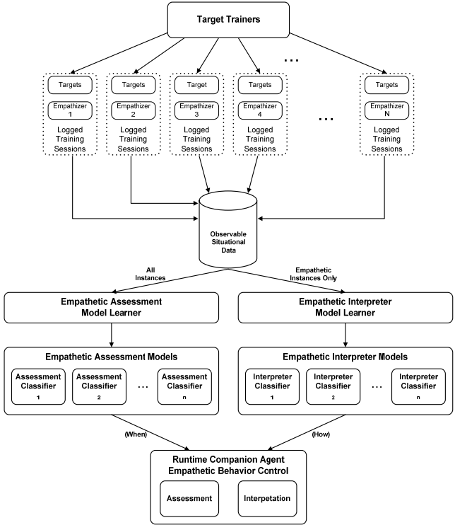
Figure 4: CARE Framework Data Flow.
