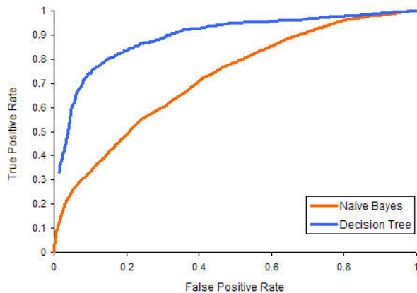
Figure 7: Empathetic Assessment (When) ROC Curves. The ROC curves for each model predicting empathetic behavior triggers in a ten second interval. The area under the naïve Bayes curve is 0.72 and the area under the Decision Tree curve is 0.89.
