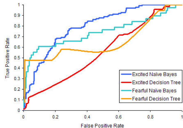
Figure 8: Empathetic Interpretation (How) ROC Curves. The ROC curves represent naïve Bayes and decision tree models for empathetic interpretation for the affective states excited and fearful . Areas under each curve are as follows: 0.80 (Excited Naïve Bayes), 0.56 (Excited Decision Tree), 0.74 (Fearful Naïve Bayes), and 0.66 (Fearful Decision Tree).
