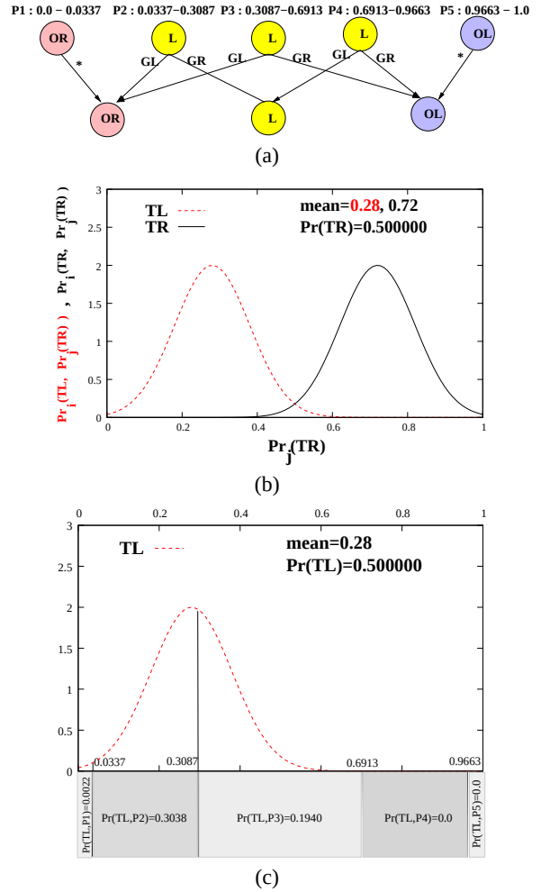
Figure 2: (a) Agent j 's horizon 2 policy showing optimal plans given different prior beliefs. Since j 's belief is not nested, its prior belief is given as the probability that the tiger is behind the right door. (b) An example of agent i 's level-1 belief. Note that we have 2 distributions, one when the tiger is on the left and other when tiger is on the right. In the belief shown, i thinks that j is likely to be somewhat informed about the tiger's true location. (c) Shows how agent i 's belief b_{i,1} \in \Delta(IS_{i,1}) (at 2 steps to go) is transformed into a belief \tilde{b}_{i,1} \in \Delta(ECIS_{i,1}) . For example, the probability that the tiger is behind the left door and j 's belief is in region P2 is given as \tilde{b}_{i,1}(TL, P2) = \int_{0.0337}^{0.3087} b_{i,1}(TL, Pr_j(TR)) dPr_j(TR) = 0.3038 , where b_{i,1}(TL, Pr_j(TR)) is the Gaussian pdf describing i 's belief about j 's belief when the tiger is on the left. \int_0^1 b_{i,1}(TL, Pr_j(TR)) dPr_j(TR) gives i 's belief that the tiger is behind the left door. Similarly, \tilde{b}_{i,1}(TR, P1), \tilde{b}_{i,1}(TR, P2) \dots \tilde{b}_{i,1}(TR, P5) are computed from the Gaussian describing i 's belief about j 's belief when the tiger is behind the right door.
