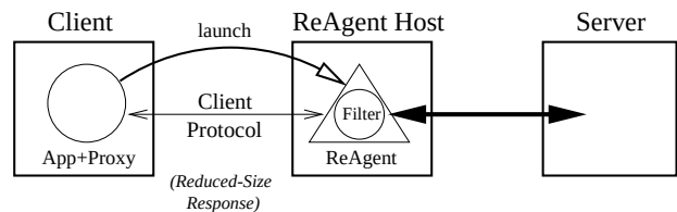
Figure 6: The Filter Behavior
