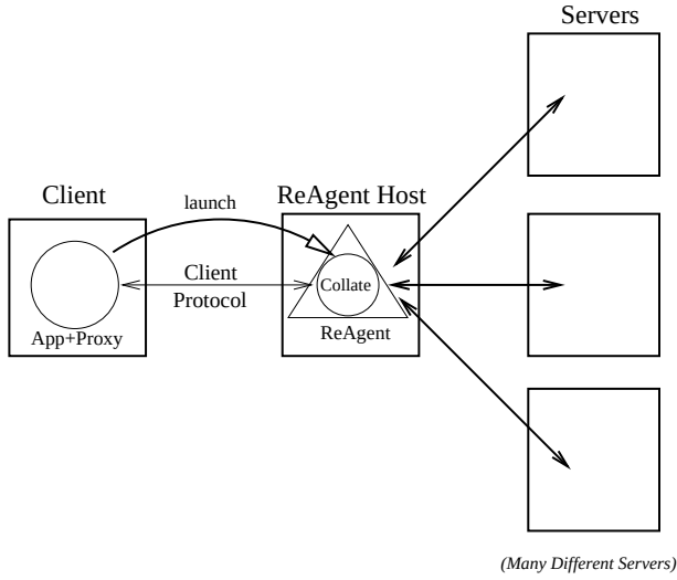
Figure 9: The Collator Behavior
