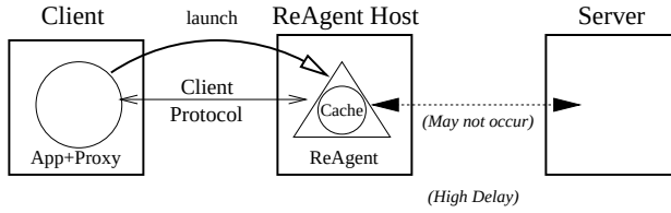
Figure 8: The Cacher Behavior
