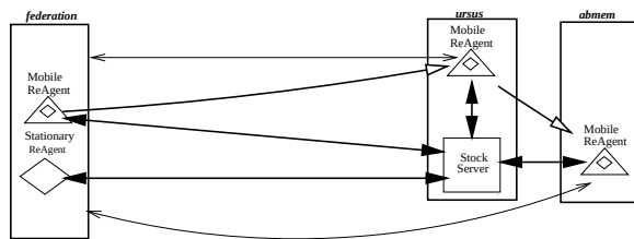
Figure 10: Stock Traders Setup
