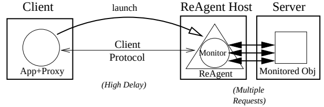
Figure 7: The Monitor Behavior
