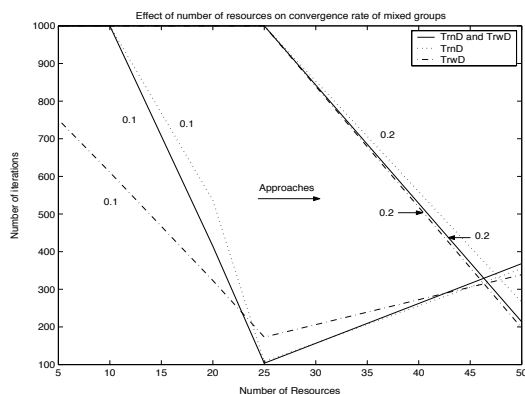
Figure 3: Speed of convergence with varying resources: 100 Agents, \gamma_k = 0.7 , \alpha = 0.1 , 0.2 .
