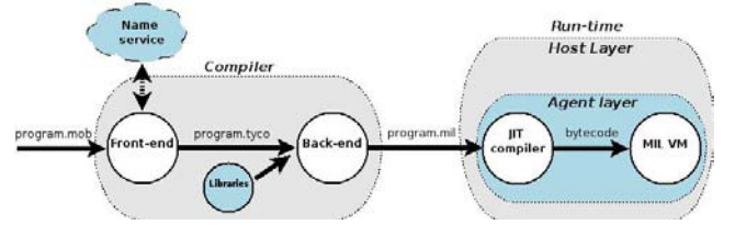
Figure 2: Compiling and running a Mob program.
