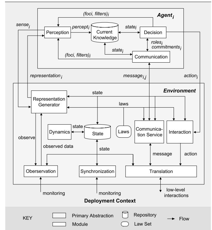
Figure 1: High-level overview of the reference architecture for situated multiagent systems
