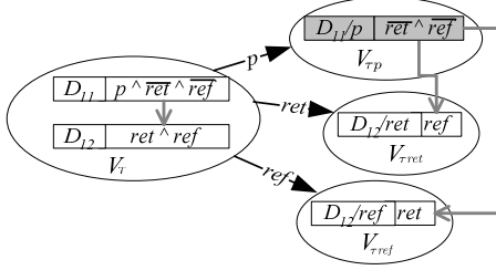
Figure 5: Clear choice: An agent can unambiguously decide which path to choose, since the evolution node preference graph has exactly one node V_{tp} , over which no other node is preferred.
