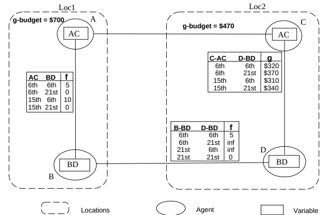
Figure 2: Meeting Scheduling Example
