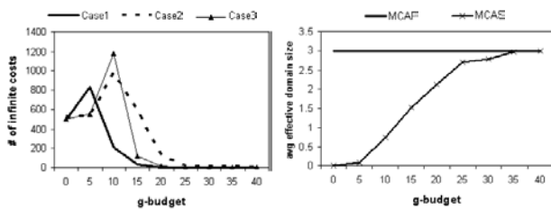
Figure 9: a) g-budget vs. number of infinite cost messages b) g-budget vs. number of values per domain
