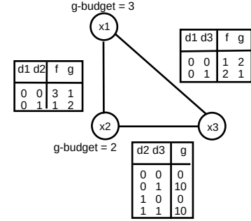
Figure 7: MCASA fails on non-T-nodes
