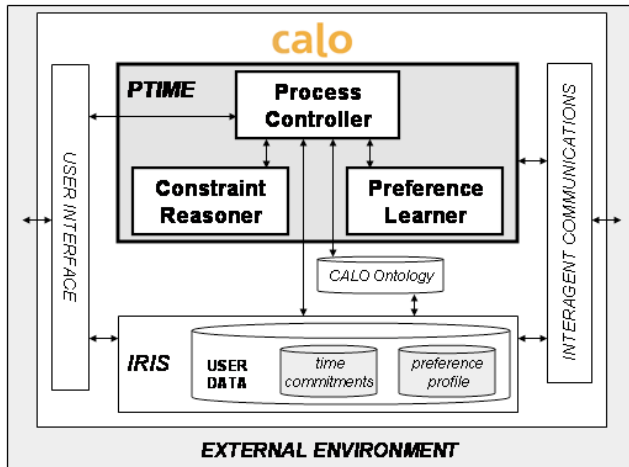
Figure 1: Architecture of a PTIME Agent
