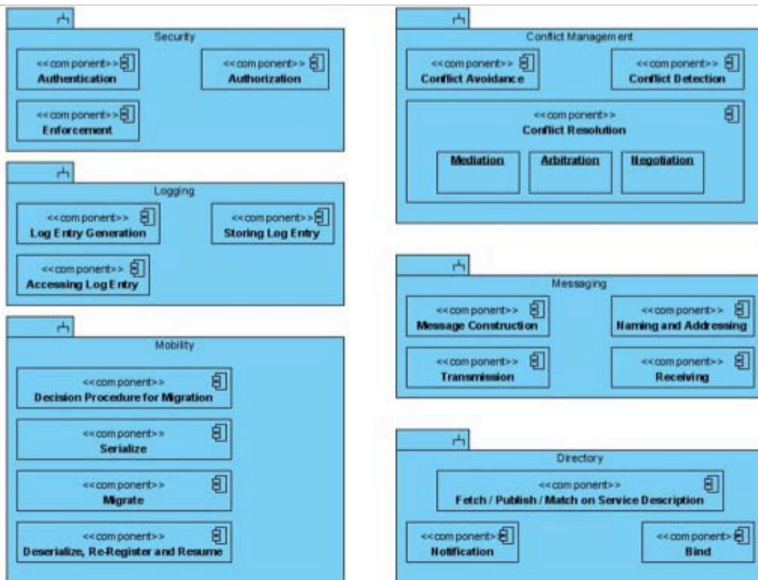
Figure 4: A Functional View of an Agent-Based System. selected functional concepts shown here in standard UML notation.
