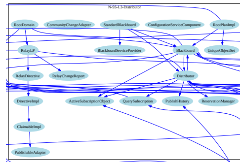
Figure 2: Diagram of Cougar's Blackboard Distributor obtained using the Bunch reverse engineering tool.
