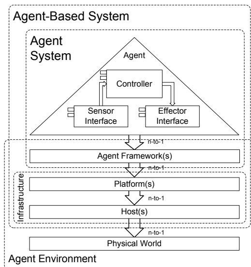
Figure 3: An Agent-Based System is made up of layers.
