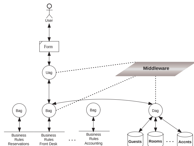
Figure 2: The middleware supervises business rules (Bag) and data base (Dag) Server Agents that handle all specialized tasks to serve the requirements of User Agents (Uag)
