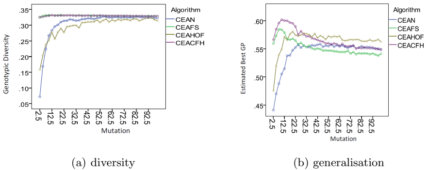
Fig. 2. Profile plots of diversity and best generalisation performance (mean over the final 60 generations) versus mutation rate for each of the 4 algorithm variants.
