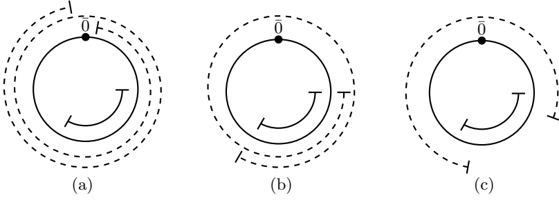
Fig. 5. (a) When the concrete range covers the entire circumference of the number circle, the proximity bounds cannot be reduced further. (b) The concrete bounds can, however, be reduced to the next corresponding proximity bound. (c) If both sets of endpoints are mutually contained, there can be no reduction.
