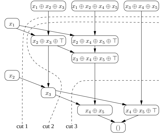
Figure 3. A xor-refutation.
