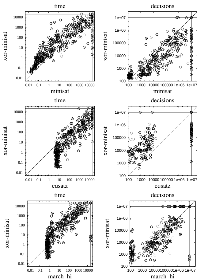
Figure 4. Results on the trivial benchmark set.
