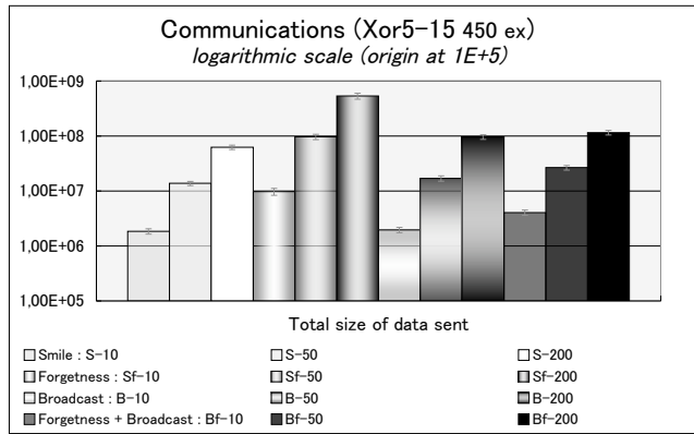
Figure 3. Communication Cost
