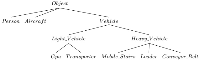
Figure 6: Tree structured object type hierarchy in the airport apron domain.
