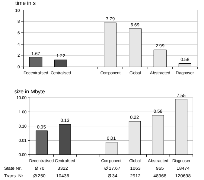
Figure 5. At the top: average diagnosis times for our models (left) and for the symbolic models presented in [10] (right), based on 100 scenarios consisting each of a sequence of 10,000 observations. At the bottom: corresponding model sizes.
