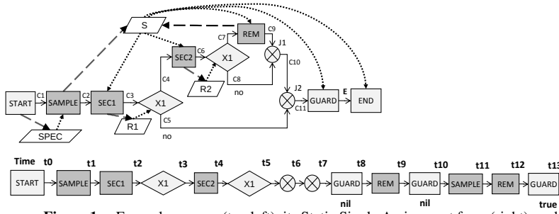
Figure 1. Example process (top left), its Static Single Assignment form (right), and a sequence of activity executions (bottom)
