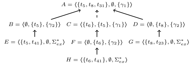
Figure 2. The full argumentation tree \mathcal{T}_1 .
