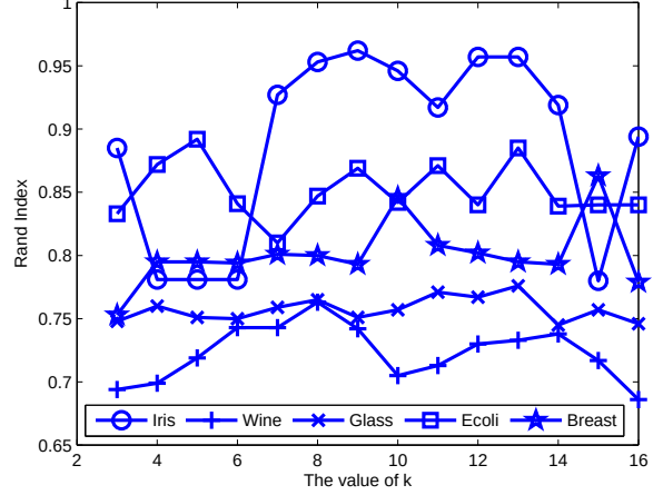
Figure 3. Rand Index measure of our approach with ASC score for some datasets using 50 queries vs. the number of neighbors k in the k -NNG
