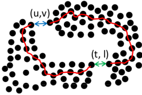
Figure 2. Illustration of the propagation mechanism: Label(t, l) is propagated as Label(u, v) because of the presence of strong paths SP(u, t, \theta) and SP(v, l, \theta) between them
