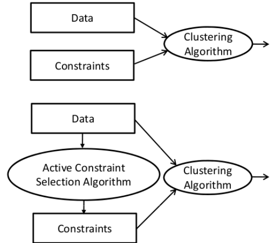
Figure 1. Illustration of passive definition of constraints (top) and active constraints learning (bottom)
