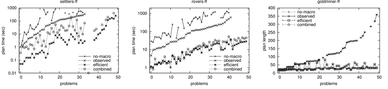
Figure 10. Sample performance: left 2 columns for plan-time, right column for plan-length; missing points: not solved
