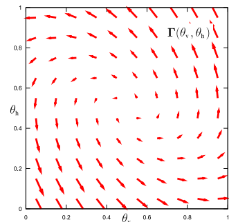
Figure 5. LPF for the Inverted two-step
