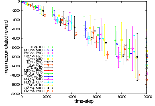
Figure 7. Average Rewards for g_v in Inverted two-step game.
