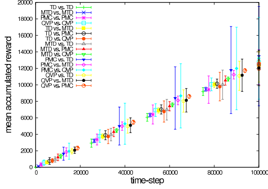
Figure 6. Average Rewards for g_v in Bowling two-step game.
