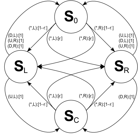
Figure 1. The Bowling two-step game as a SMAFASP.
