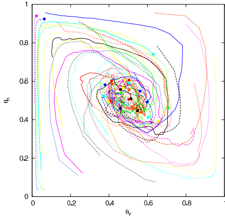
Figure 8. TD versus TD in Bowling two-step game
