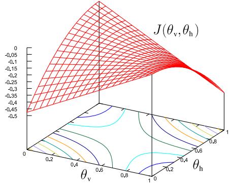
Figure 3. J_h for Bowling two-step game
