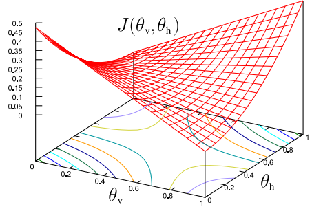
Figure 2. J_v for Bowling two-step game
