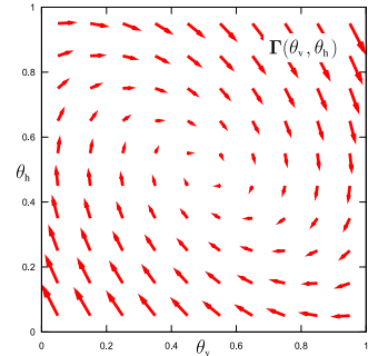
Figure 4. LPF for the Bowling two-step
