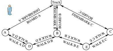
Figure 2. A domain transition graph for the driver variable from the example in Figure 1.
