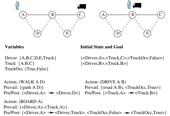
Figure 1. A simple planning problem, and the corresponding SAS + representation, used as a running example. The initial state is shown to the top-left and the goal state to the top-right.
