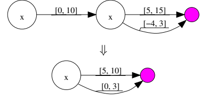
Figure 4. Merging of stammering nodes.
