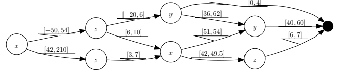
Figure 2. An example of focusing interval automaton. Variable domains are as follows: \text{Dom}(x) = [0, 100] , \text{Dom}(y) = [0, 100] and \text{Dom}(z) = \{0, 3, 7, 10\} .
