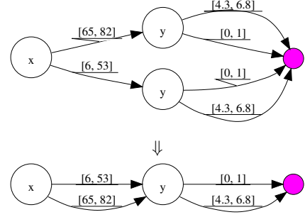
Figure 3. Merging of isomorphic nodes.
