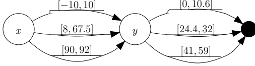
Figure 1. An example of interval automaton. Its model set (see Definition 2), represented as a union of boxes, is [-10, 10] \times [0, 10.6] \cup [-10, 10] \times [24.4, 32] \cup [-10, 10] \times [41, 59] \cup [8, 67.5] \times [0, 10.6] \cup [8, 67.5] \times [24.4, 32] \cup [8, 67.5] \times [41, 59] \cup [90, 92] \times [0, 10.6] \cup [90, 92] \times [24.4, 32] \cup [90, 92] \times [41, 59] .
