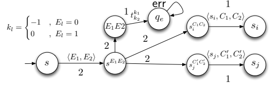
Figure 3. Construction used in the proof of Theorem 4 for (s, E_1, E_2) \Delta (s_i, C_1, C_2) and (s, E_1, E_2) \Delta (s_j, C'_1, C'_2) .
