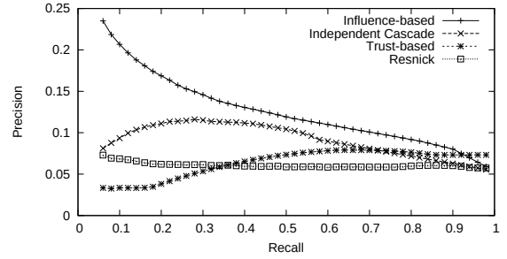
Figure 5. Precision-recall curve
