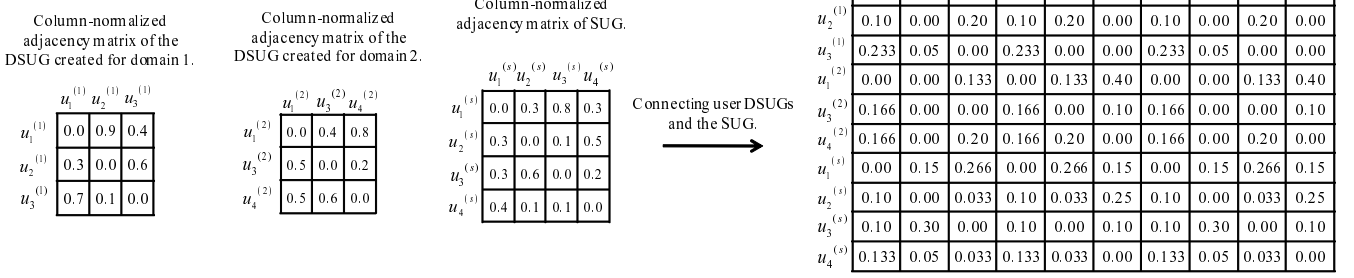
Figure1. Example of creating the column-normalized adjacency matrix of the CDUG.
