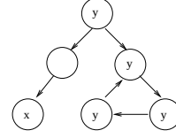
Figure 1. A counterexample for AG\neg x \vee AF\neg y .
