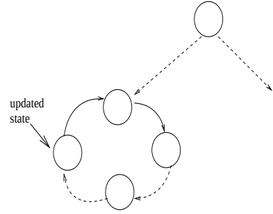
Figure 4. A case of update with \text{AF}\phi .
