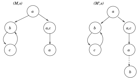
Figure 3. Updating (M, s) with \text{A}[a\text{U}(\neg a \wedge b)] \vee \text{AX}a preserves the persistence of \text{AFAX}(a \vee c) .
