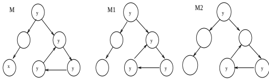
Figure 2. Updating (M, s) with \text{AG}\neg x \vee \text{AF}\neg y .
