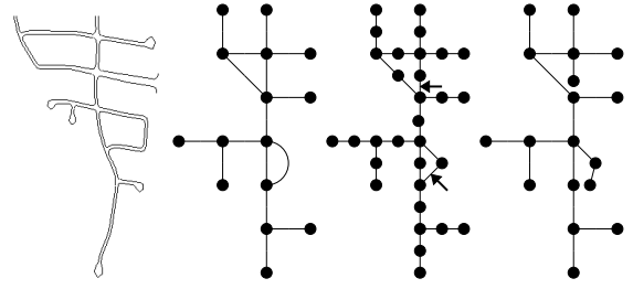
Figure 1. Small subdivision (left); multigraph (middle left); augmented graph (middle right) with two edges marked by arrows for removal to form a spanning tree; cut graph (right).
