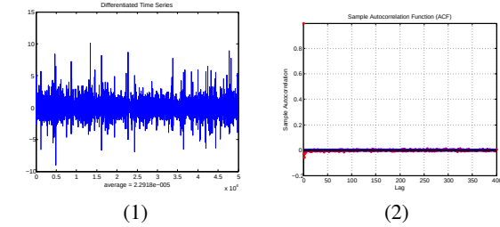
(b) Differentiated wind speed time series and autocorrelation. (1) Differentiated wind speed time series, (2) Autocorrelation of differentiated time series
