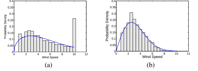
Figure 2: Fit Wind Speed time series data with a single Weibull distribution. (a) Fitted PDF (blue line: 2-parameter Weibull) of the NY-ISO dataset (b) Fitted PDF of the IL-ISO dataset. Both null hypotheses are declined at the significance level 0.05 use Anderson-Darling test.
