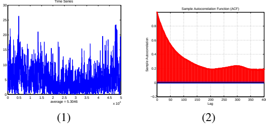
(a) Wind speed time series and autocorrelation. (1) Wind speed time series, (2) autocorrelation
