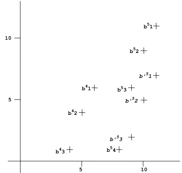
Figure 5. Path b -costs for D_4 and D_5 .
