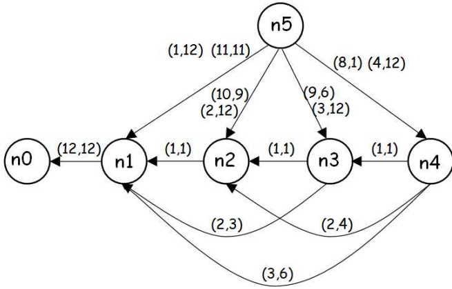
Figure 3. The graph D_5 .
